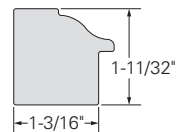
BACK BAND #7931C16
