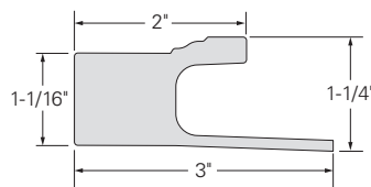
J-CHANNEL BRICKMOULD #5657P17
