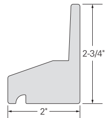
WATER TABLE #5170C18
