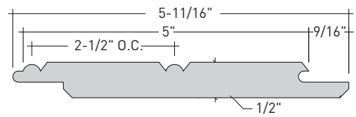
6" KLEERLOK® BEADED BOARD
