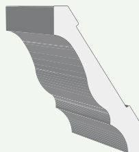
3-5/8" CROWN MOULDING #5049P16
