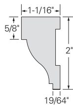
RAKE MOULDING #5287P16
