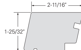
LARGE HISTORIC SILL #7435C16
