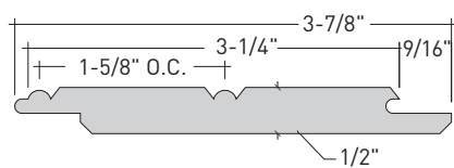
4" KLEERLOK® BEADED BOARD
