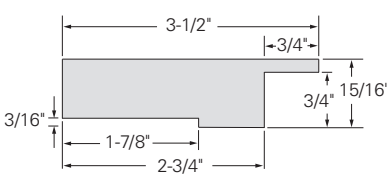
KLEER KONCEAL® TRIMBOARD WITH NAILING FLANGE CUTOUT
